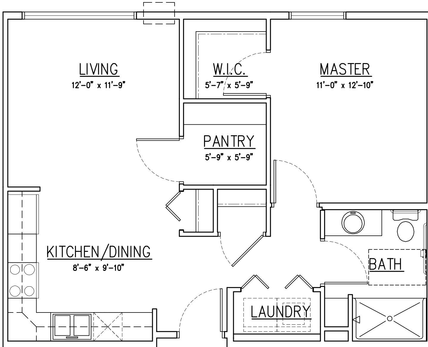
UNIT PLAN - 1A
